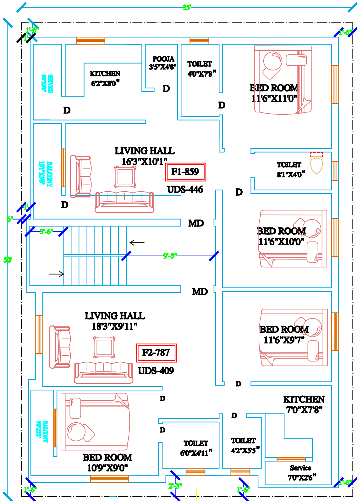
FIRST FLOOR
